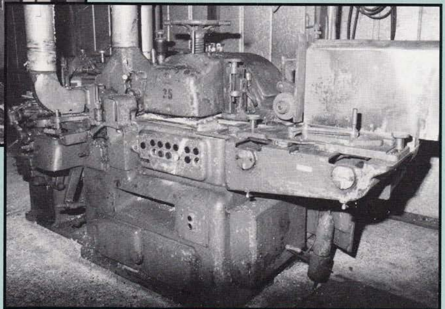
Mattison 276 moulder (1 of 2)
